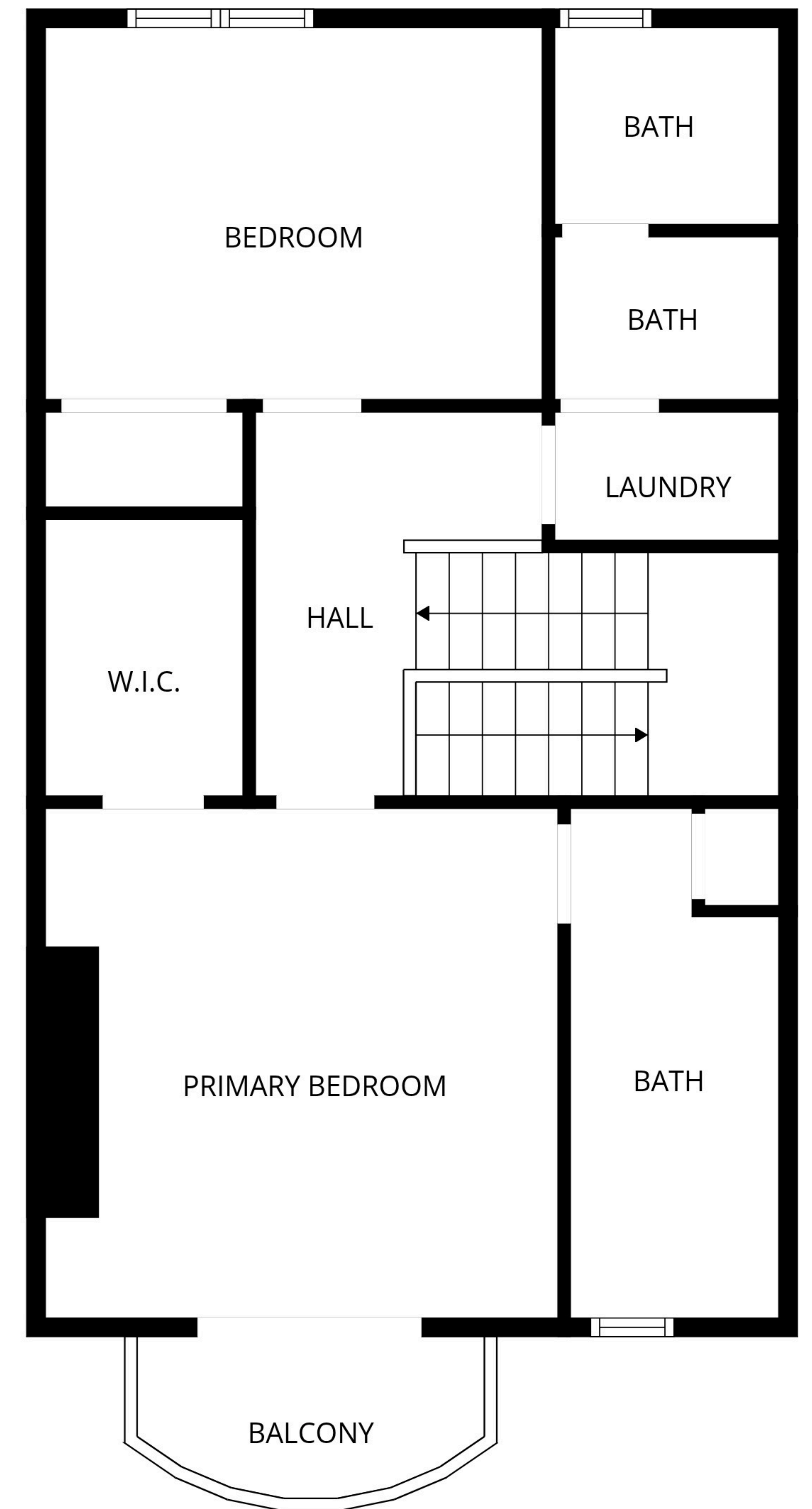
FLOOR 3
