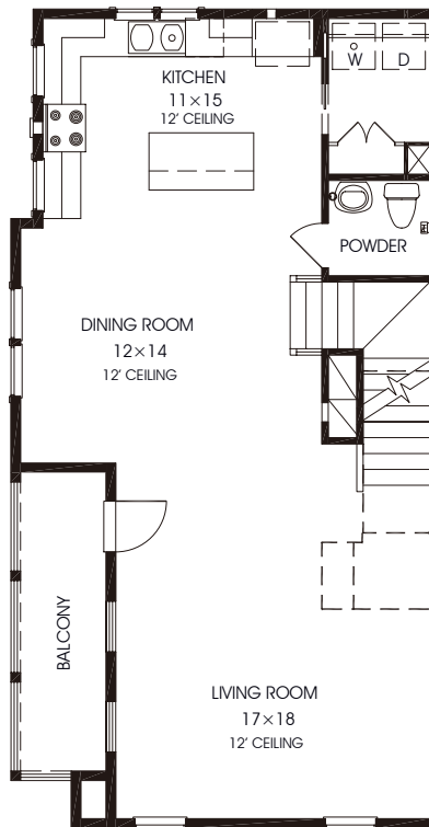
Second Floor 861 sq.ft.
