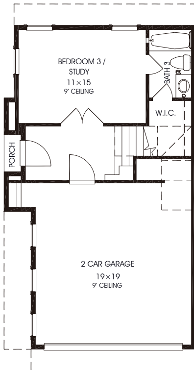
First Floor 369 sq.ft.
