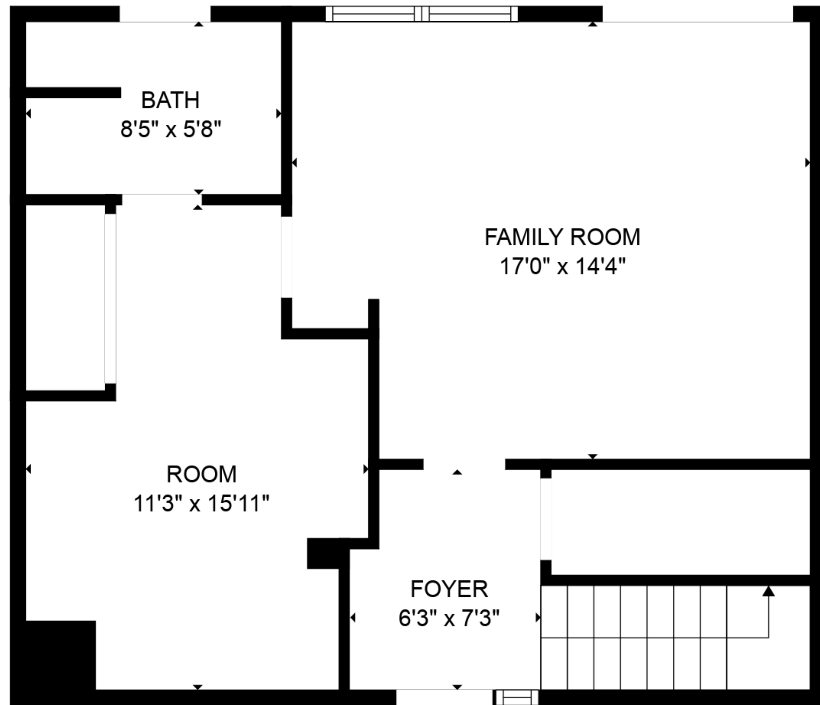
FLOOR 1
