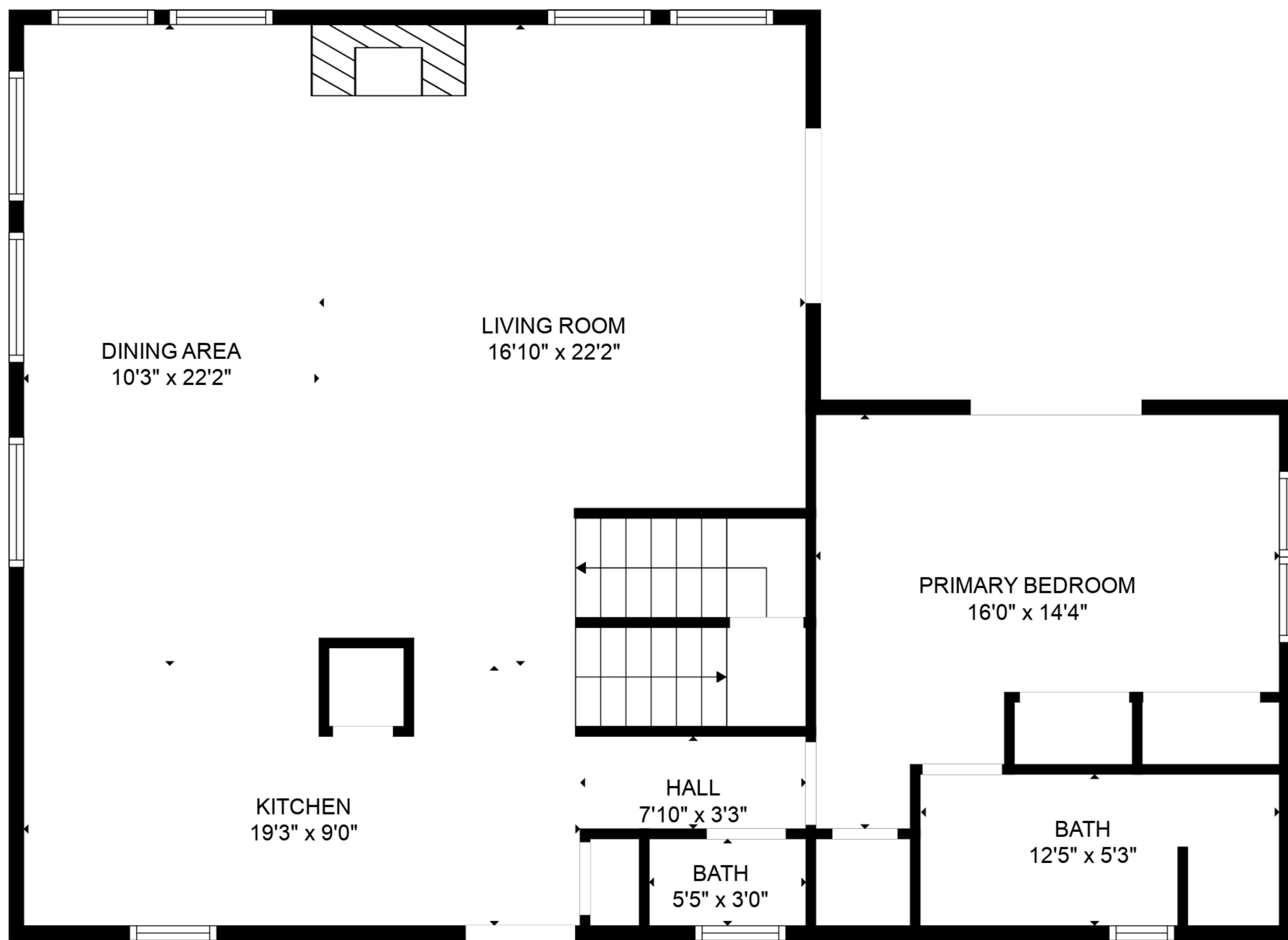
FLOOR 2
