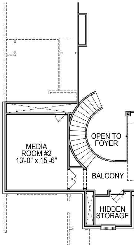
SECOND FLOOR PLAN OPT. #0467 MEDIA ROOM #2 FROM ATTIC SPACE
