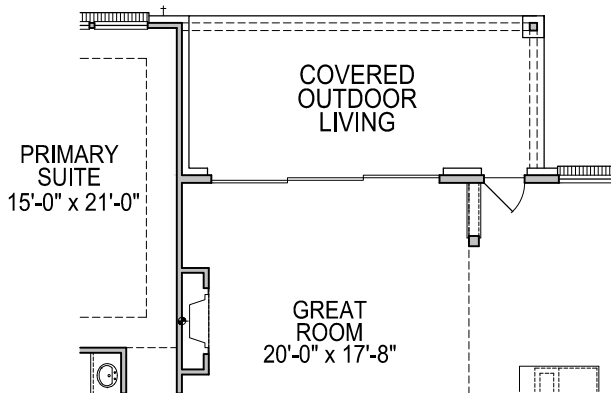
FIRST FLOOR PLAN OPT. #0790 SLIDERS @ GREAT ROOM
