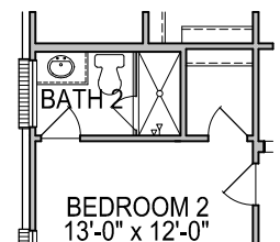
FIRST FLOOR PLAN OPT. #0486 ALT. BATH 2 LAYOUT
