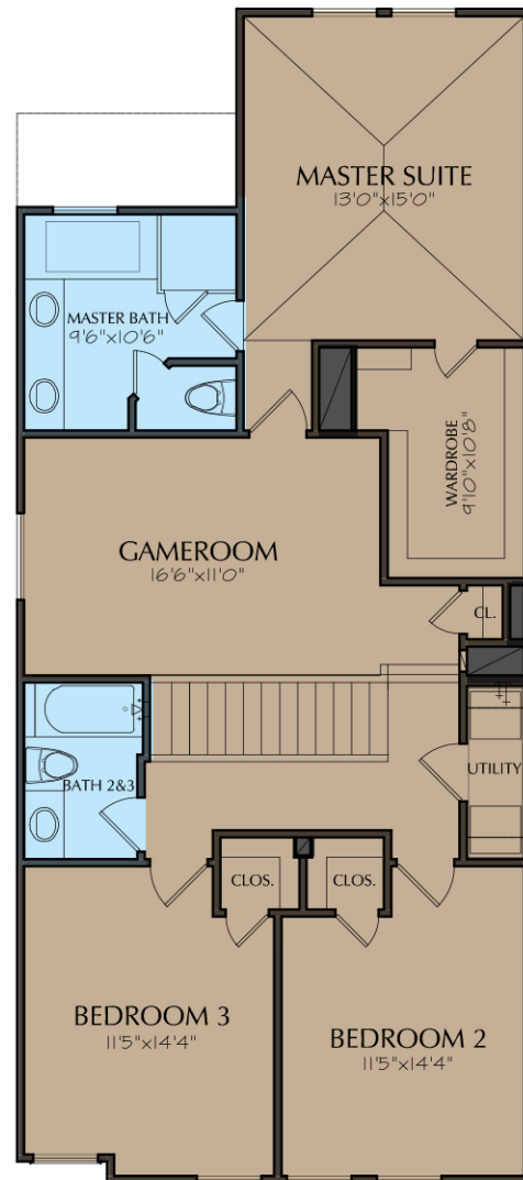
SECOND FLOOR
