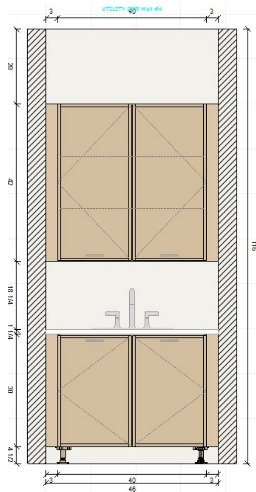
Sink Elavation
