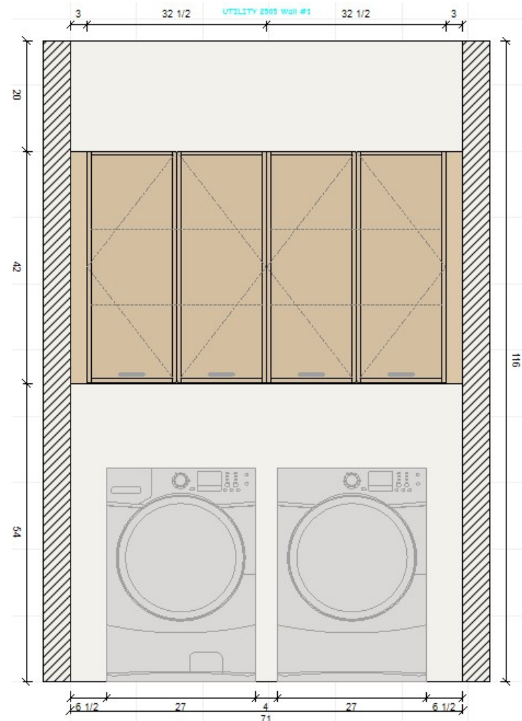
W/D Elevation
