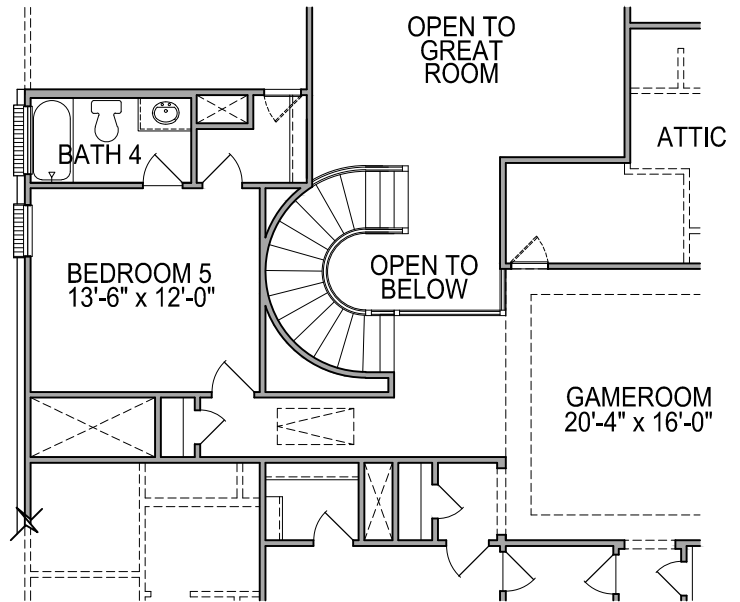
SECOND FLOOR PLAN OPT. #0094 BED5/BATH 4
