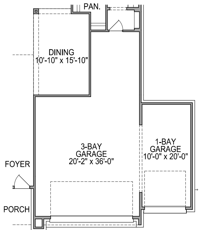
FIRST FLOOR PLAN OPT. #0593 1 BAY GARAGE EXT.
