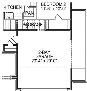
FIRST FLOOR PLAN OPT. #0613 5' GARAGE EXT.
