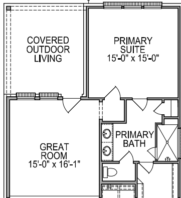
FIRST FLOOR PLAN OPT. #0105 COVERED OUTDOOR LIVING
