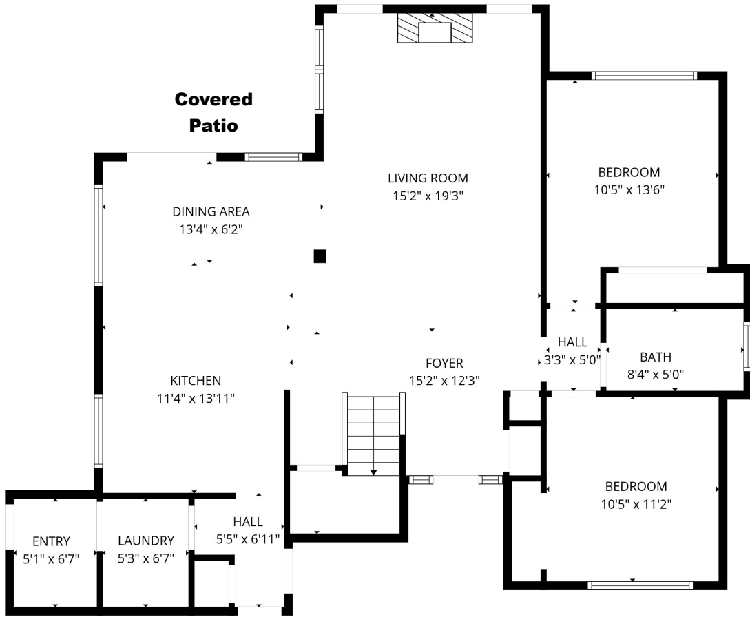
1st floor
