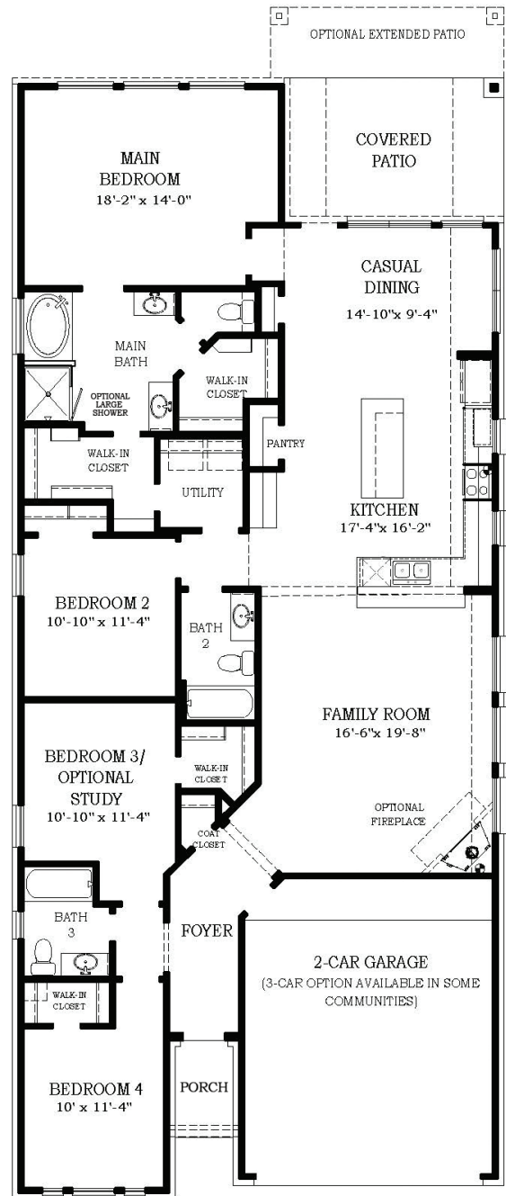
FLOOR PLAN
