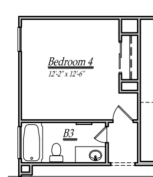
Optional Bedroom 4 & B3 Additional 178 sq/ft
