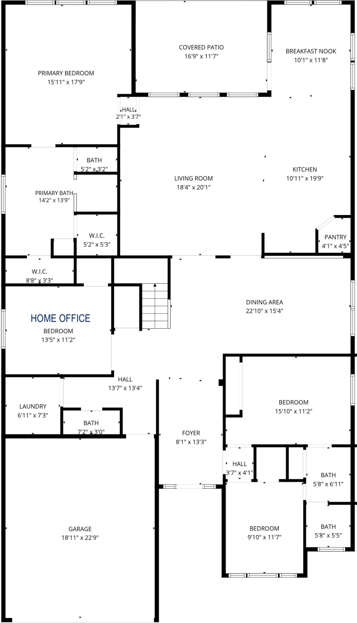
FLOOR 1
