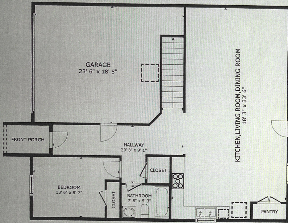
FLOOR 1
